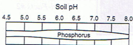
Figure 1. Effects of soil pH on P availability.
