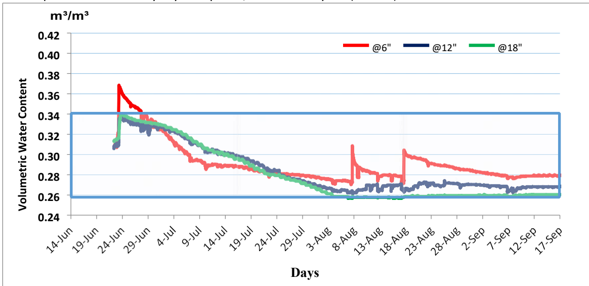
Figure 2. Volumetric water content (m 3 /m 3 ) on soybeans of On-Row treatments, NCRS, 17- 716.
