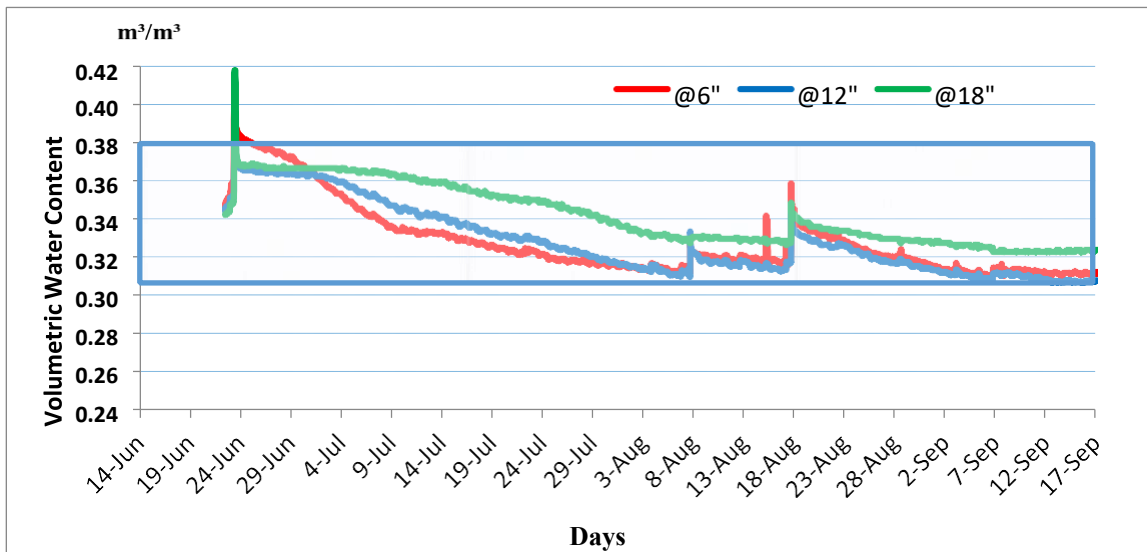
Figure 3. Volumetric water content (m 3 /m 3 ) on soybeans of Between-Row treatments, NCRS, 17- 716.
